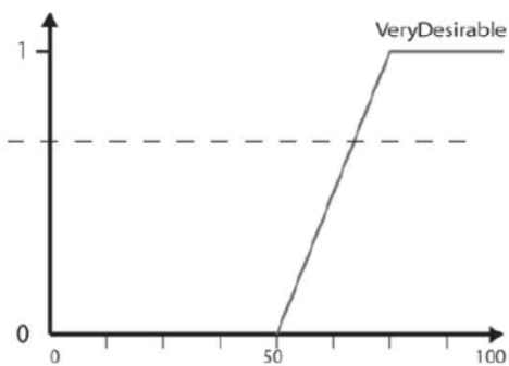
Desirability (consequent)
